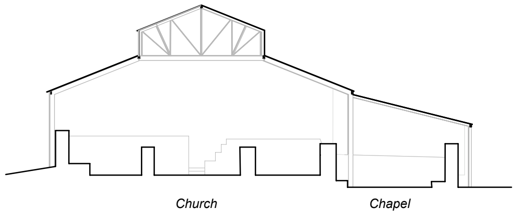
Cross-section, shelter 3
