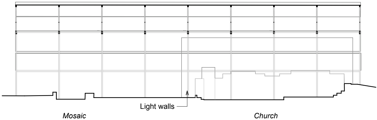
Longitudinal section, shelter 3
