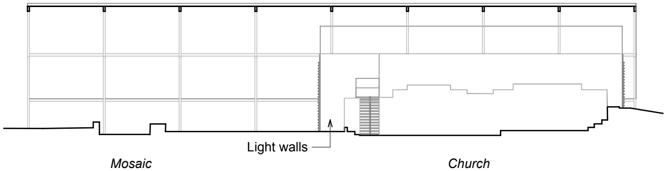
Longitudinal section, shelter 2
